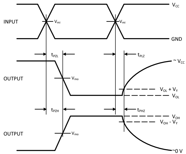
Figure 4. Switching Waveforms
