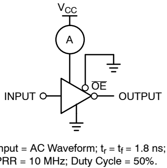
Figure 6. I_{OCD} Test Circuit
