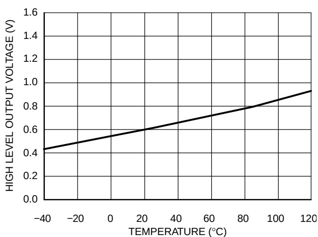
Figure 31. High Level Output Voltage vs. Temperature
