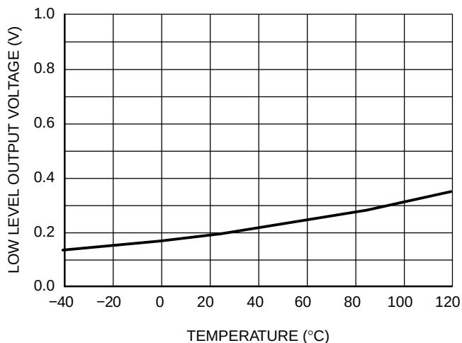
Figure 29. Low Level Output Voltage vs. Temperature
